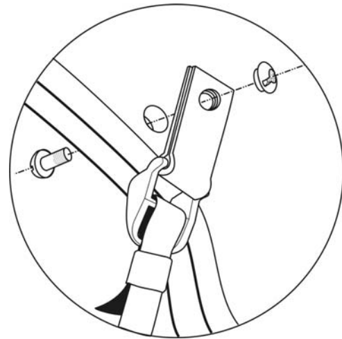
Fig 28-2 Routing of Chinstrap Webbing through Attachment Tab
