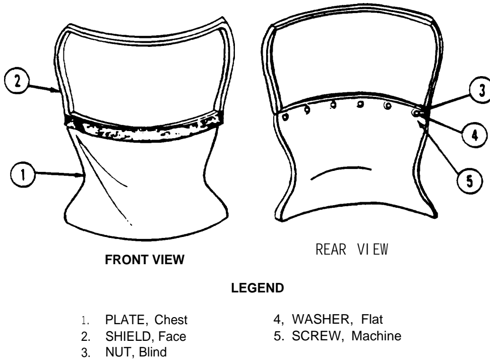
Figure 23-9. Replaceable Items on Chest Plate and Face Shield
