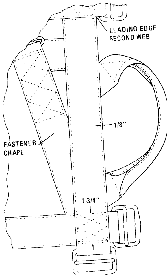
Figure 12-17. Replacement details, adapter portion of handle strap.
