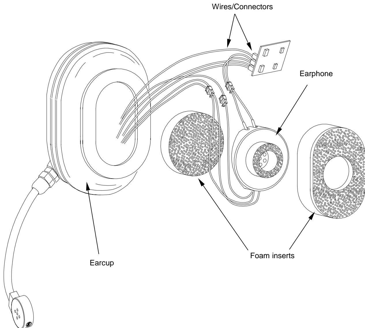
Figure 26-12. Headset Assembly
