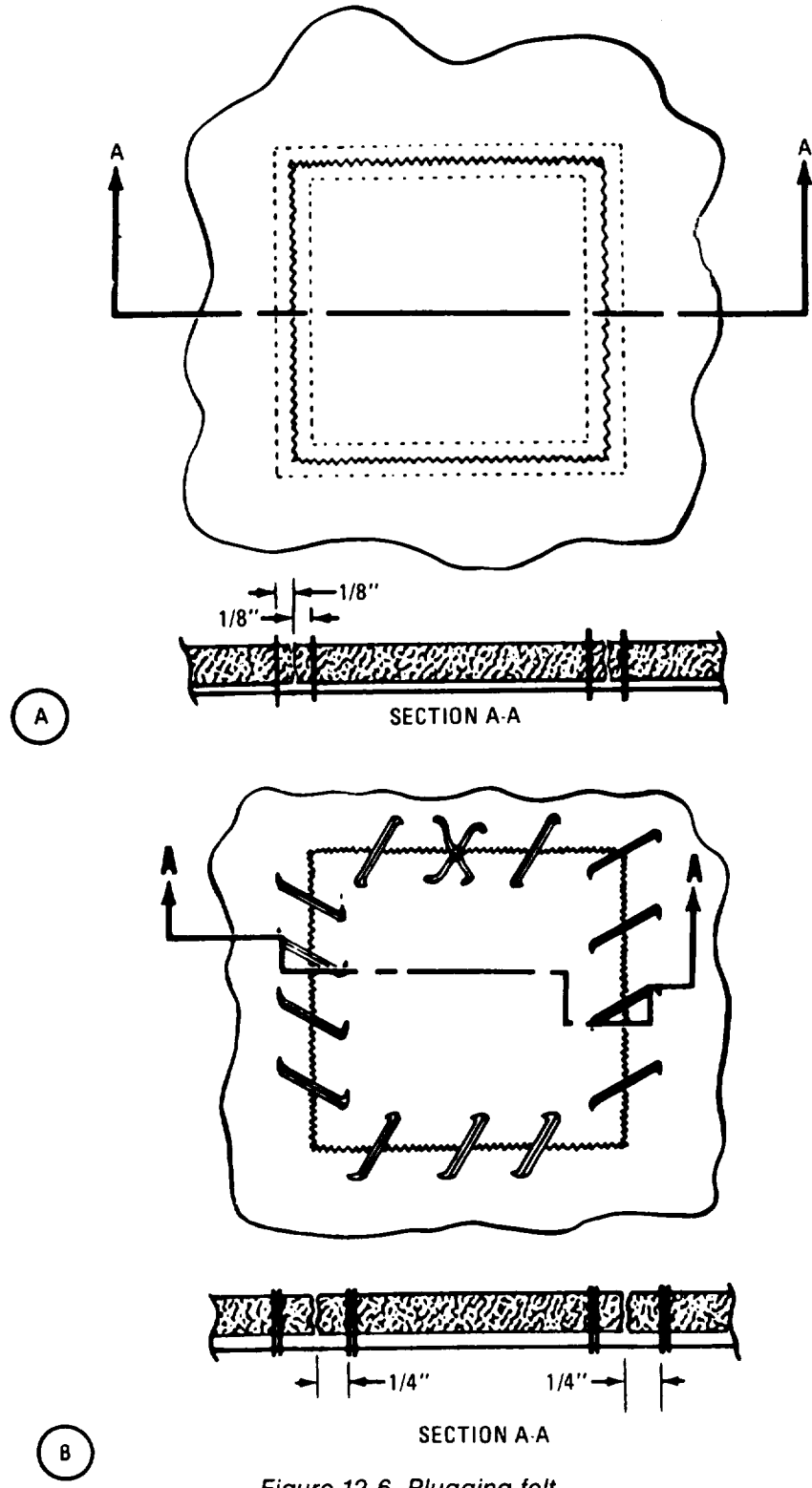
Figure 12-6. Plugging felt.
